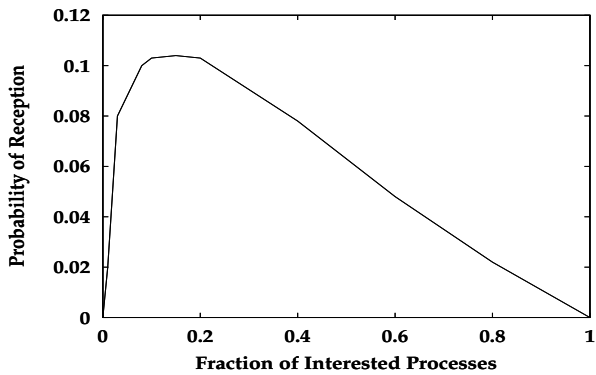
Figure 4. Infected Interested Processes; n \approx 10000 ( a = 22 ), d = 3 , R = 3 , F = 2
