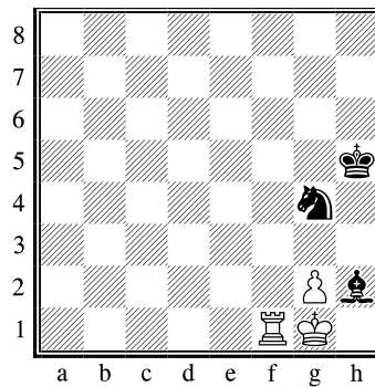
escape3: Kg1-h1
