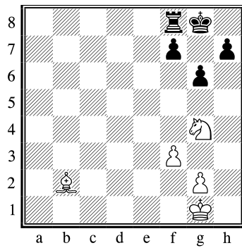
mat1_8: Ng4-h6
