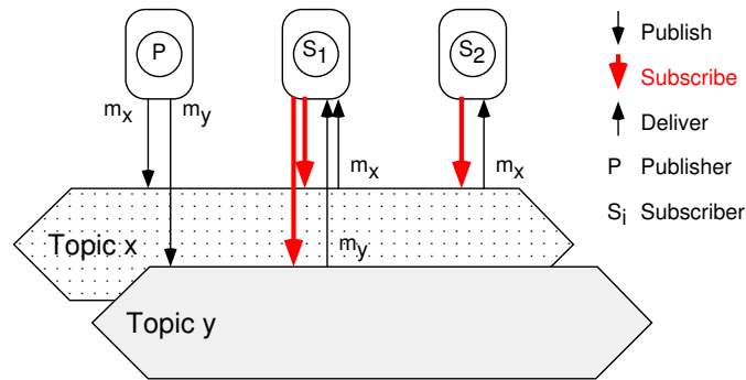
Fig. 2. Topic-Based Subscribing
